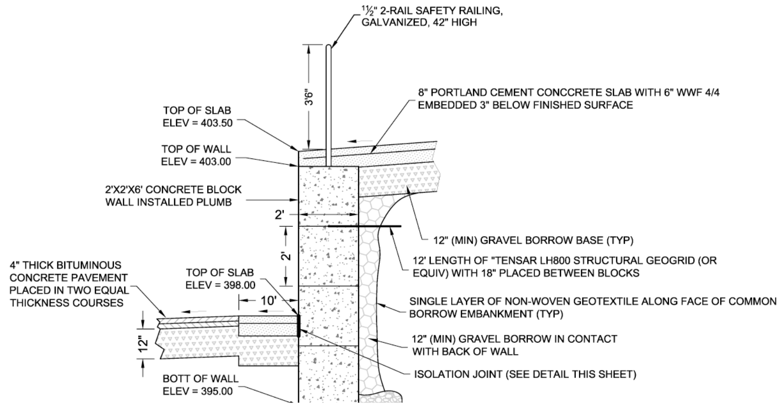
Detail of upper and lower concrete pad connections to block wall
